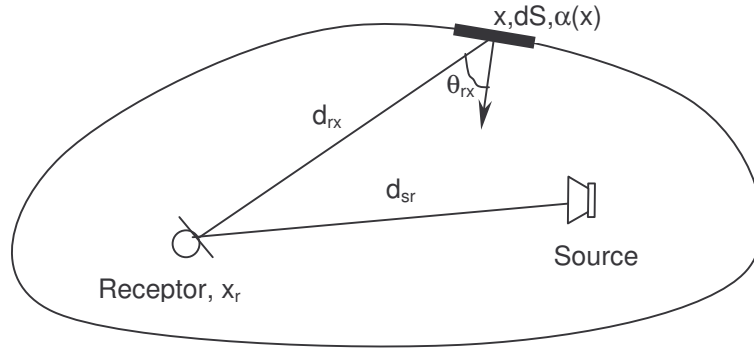
Fig. 2. Intensity received by the receptor
