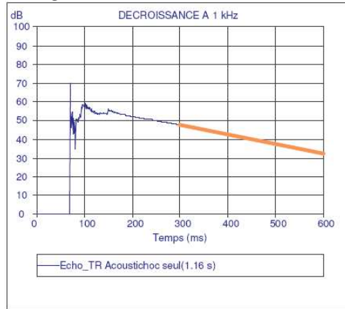
Fig. 3. Echogram at 1 kHz
