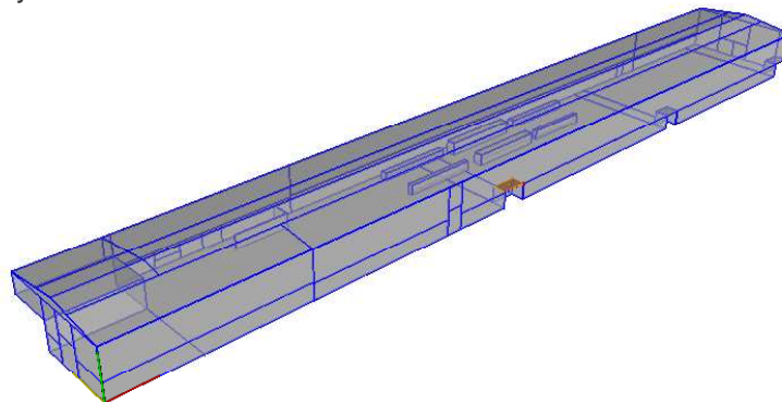
Fig. 8. modelisation of the factory
